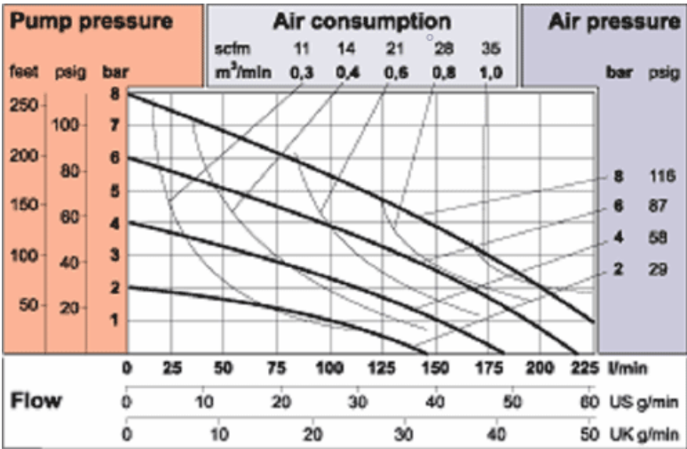
T125 - 125 l/min, 1 1/2"
