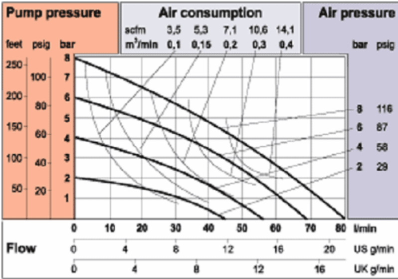
T425 - 425 l/min, 3"
