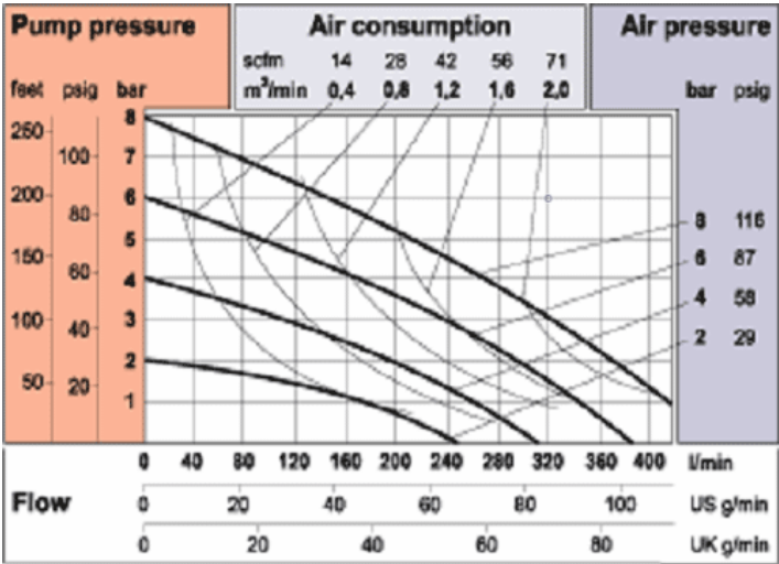
T80 - 80 l/min, 1"
