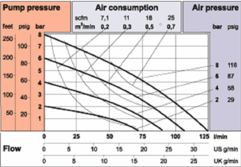
T225 - 225 l/min, 2 1/2"
