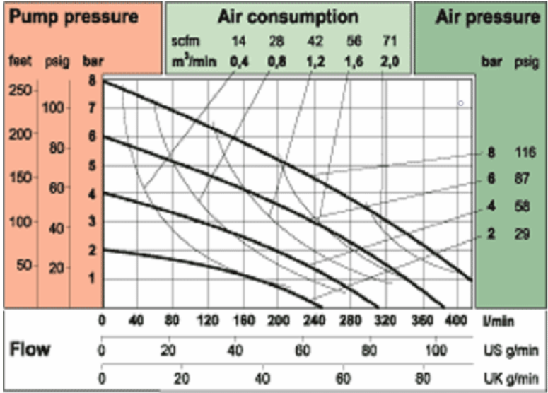
T420 - 420 l/min, 2"
