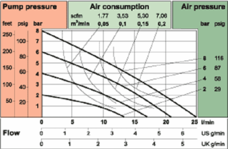
T25 - 25 l/min, 1/2"
