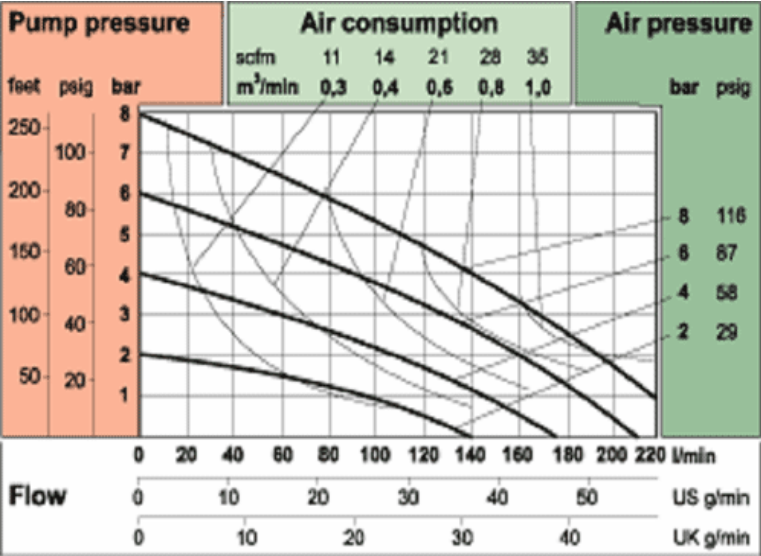
T220 - 220 l/min, 1 1/2"
