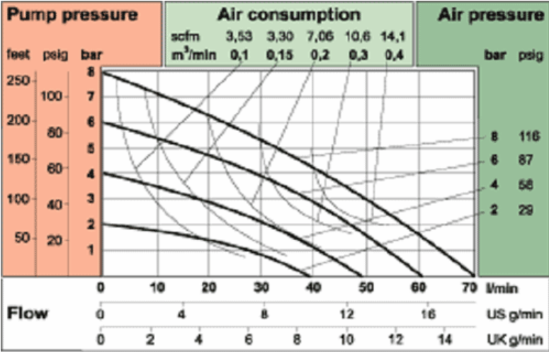
T70 - 70 l/min, 3/4"
