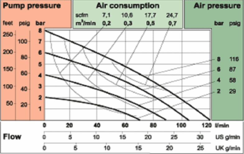
T120 - 120 l/min, 1"
