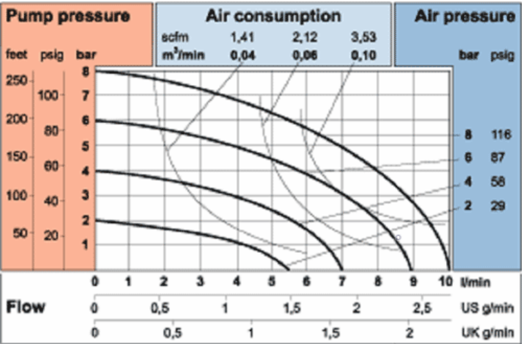
TR9 - 9 L/Min, 1/4"
