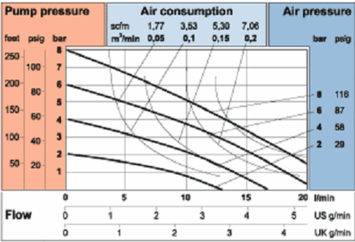
TR20 - 20l/min, 3/8"
