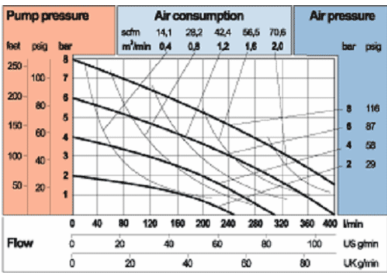
T400 - 400l/min, 2"
