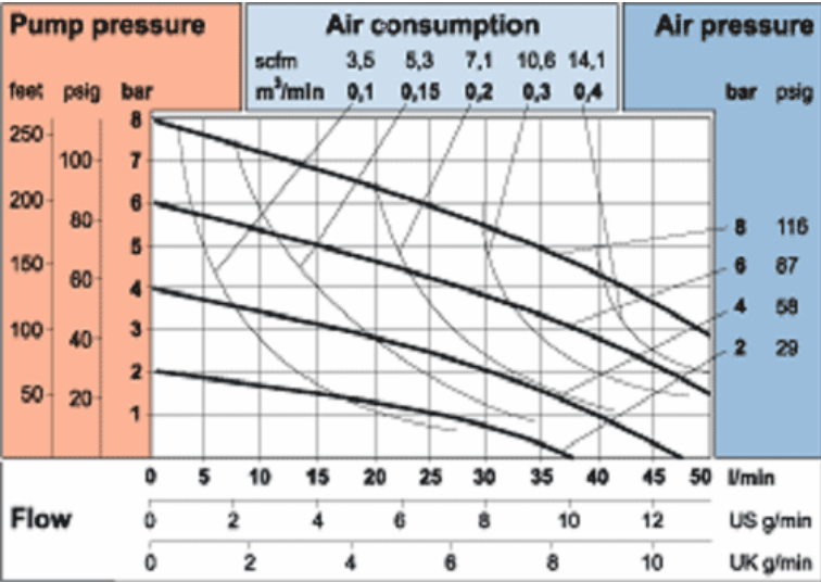
T100 - 100 l/min, 1"
